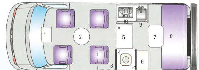
left: optional wardrobe cabinet replaces fourth seat.
